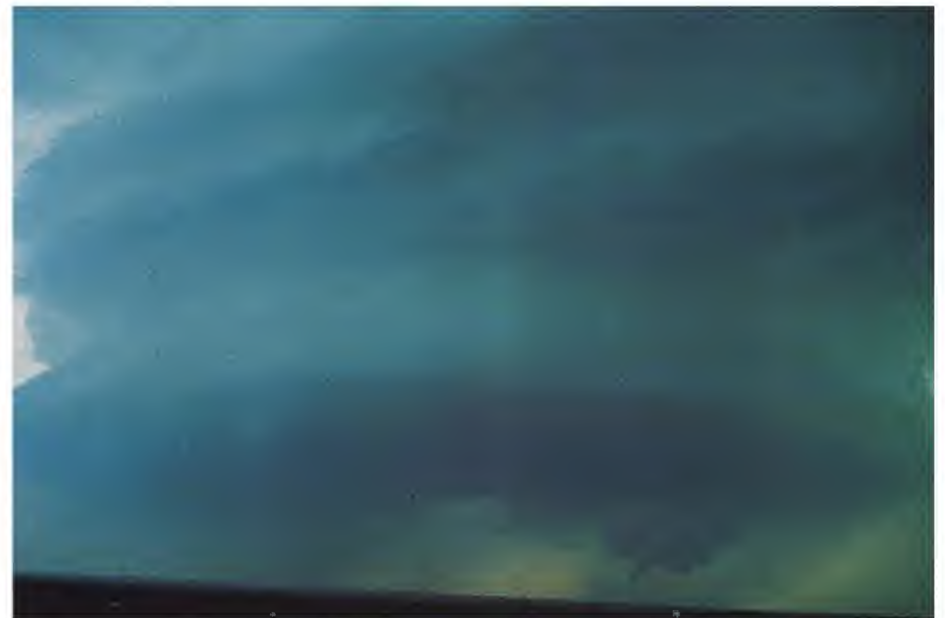
Figure 18. Striations are evident as the cork-screw-type markings on the side of this supercell updraft tower. View is to the west. Photo - Alan Moller.
